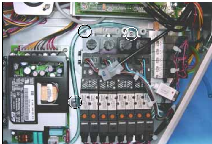
Figure 13—Pneumatic Module fastener locations. The Probe Vacuum Tubes have been disconnected.
