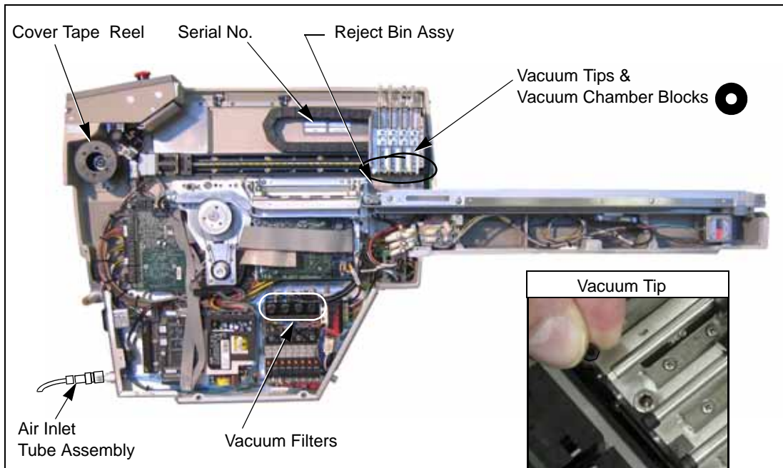
Figure 51—Parts in the Basic Spares Kit; Large Format RoadRunner
