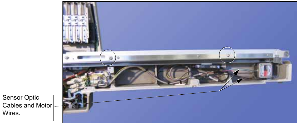
Figure 17—Location of the Mounting Screws (circled) on the Conveyor Module. Some models have SMT Adapters attached to the chassis nose. It does not need to be removed to remove the Conveyor Module.
