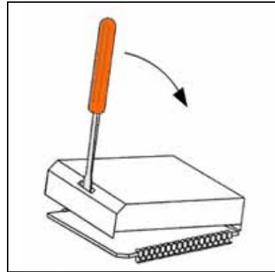
Figure 44—Removing the cap from the base.
