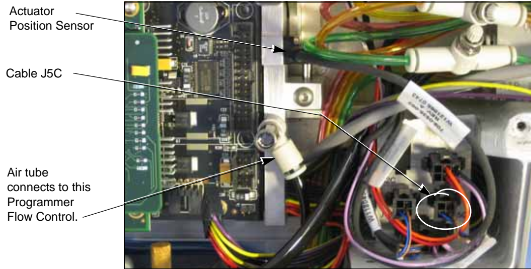
Figure 36—Cable Interconnect Panel. Cables J3 and J4 have been unplugged.
