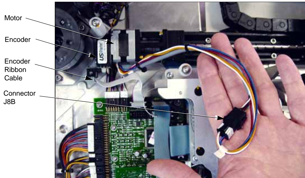
Figure 47—Wires from the Linear Stage Motor terminate at intermediate connector J8B beneath the Tape-In Module.
