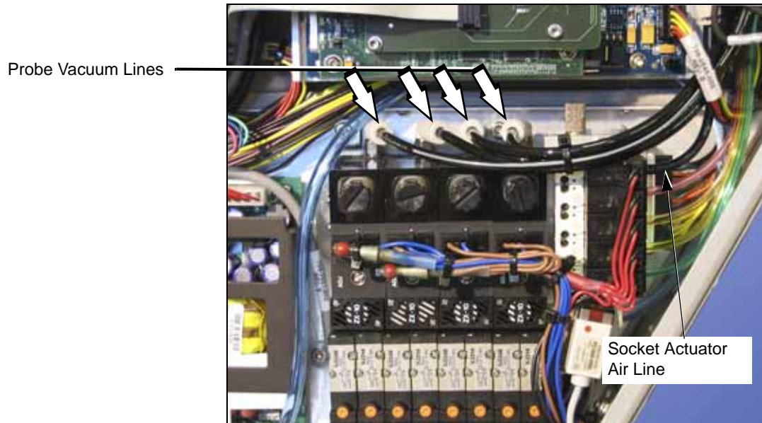
Figure 11—Location of Vacuum and Air Lines
