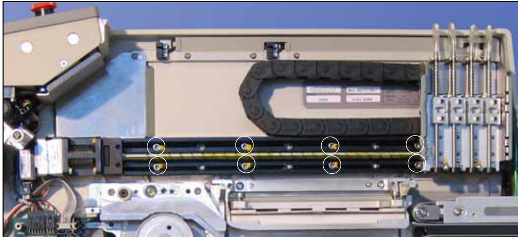
Figure 48—Linear Stage Screw Locations.
