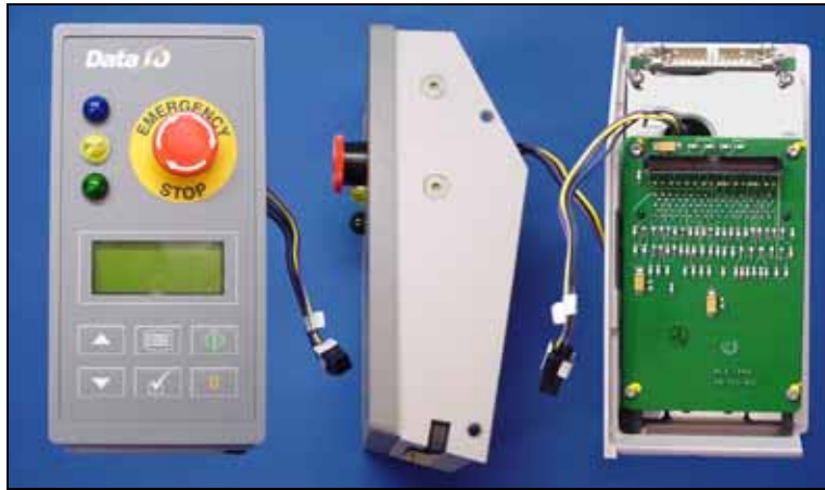
Figure 24—Control Panel Module
