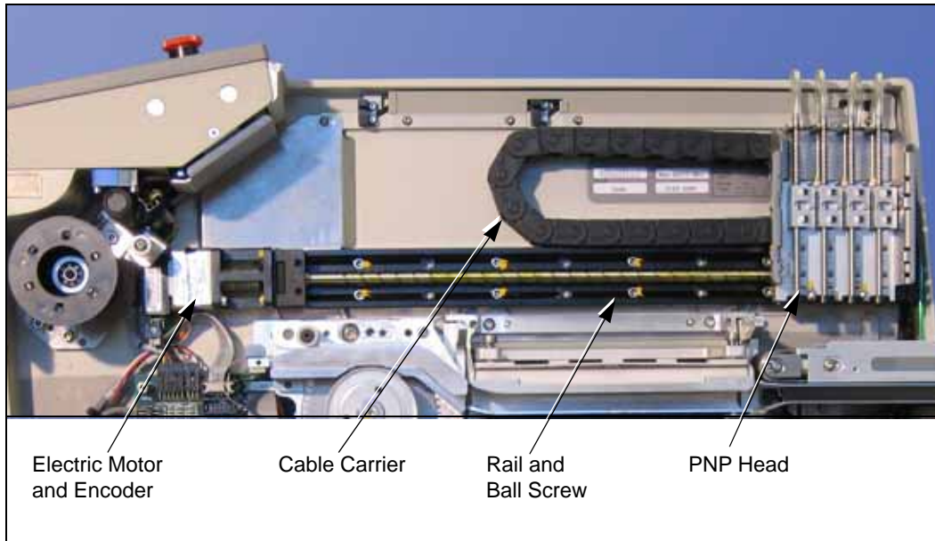
Figure 46—The Linear Stage Module
