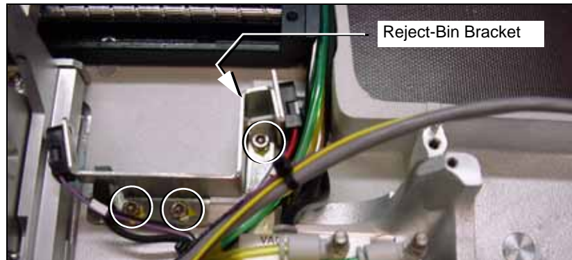
Figure 34—Reject Bin Bracket Screw Locations
