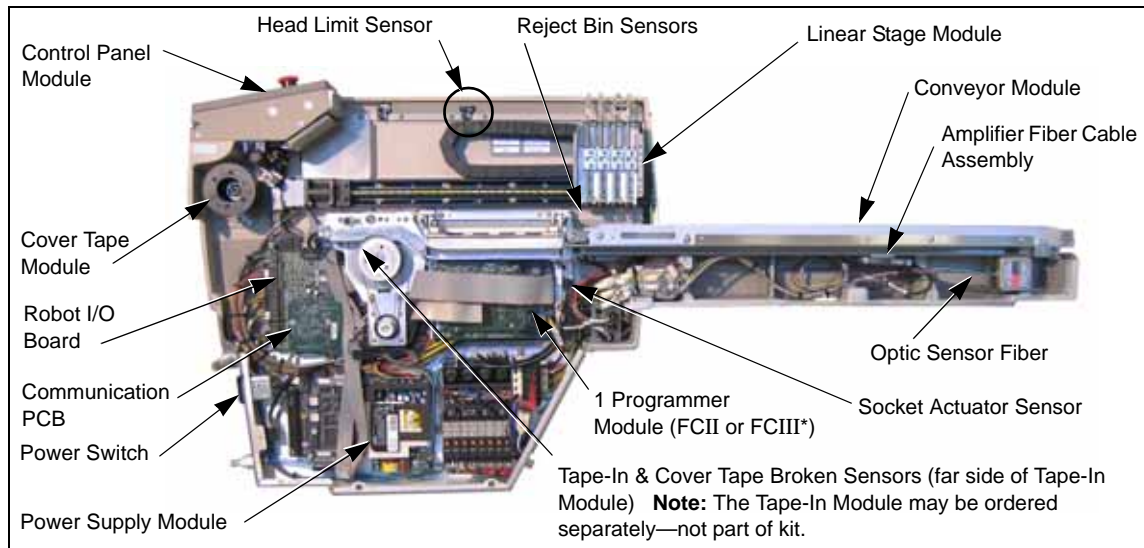
Figure 50—Parts in the Self-Service Spares Kit; Standard RoadRunner
