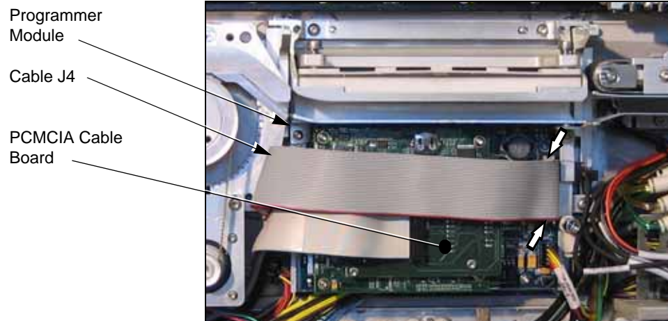
Figure 33—Programmer Module. The ribbon cable connector is indicated with two arrows.
