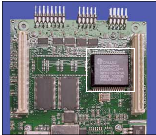
Figure 43—The PowerCap Module on the RPX-Lite PCB.
