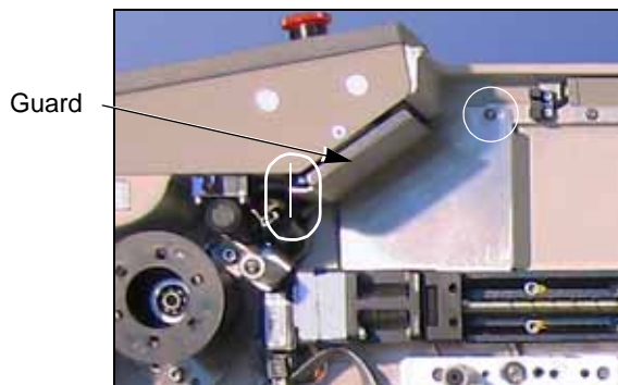
Figure 25—Ribbon Cable Guard with Screw Locations Indicated.
