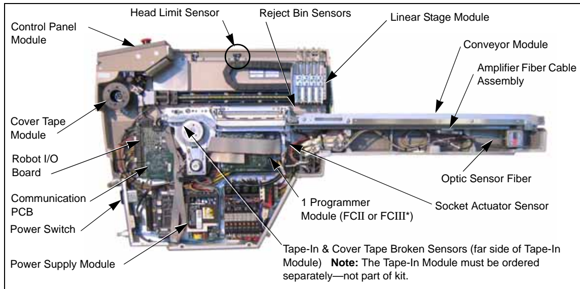
Figure 52—Self-Service Spares Kit; Large Format RoadRunner
