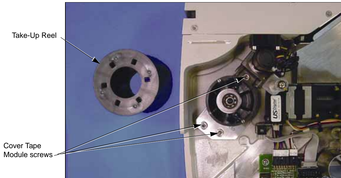
Figure 16—Location of the Cover Tape Module Mounting Screws (with the Reel Removed)
