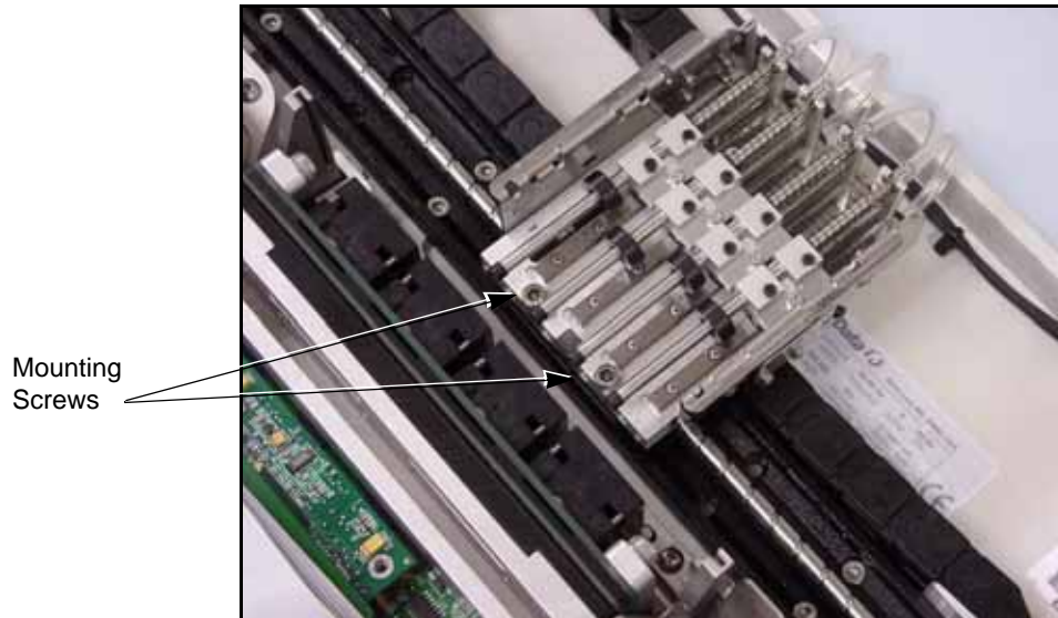
Figure 31—Removing the PNP Head
