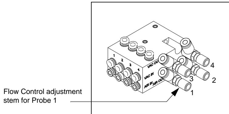
Figure 27—Interface Manifold (Adjustment stems have screwdriver slots.)
