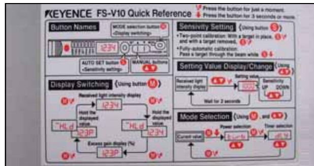
Figure 21—End-of-Belt Optical fiber Amplifier Label on the Conveyor Cover.
