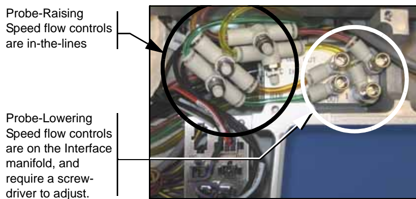
Figure 28—The in-line flow controls for adjusting the Probe Speed. Probe numbers are stamped on the manifold.
