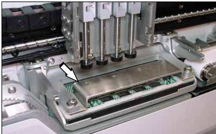
Figure 38—The Programmer Module Alignment Tool Installed on the Programmer.
