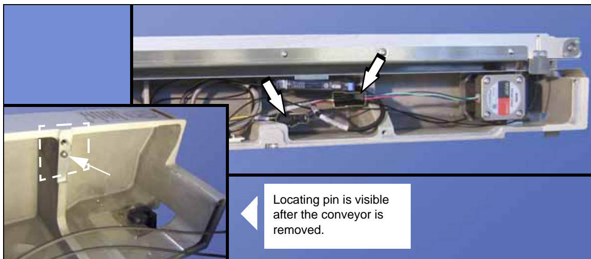
Figure 18—Conveyor Wire Connectors.
