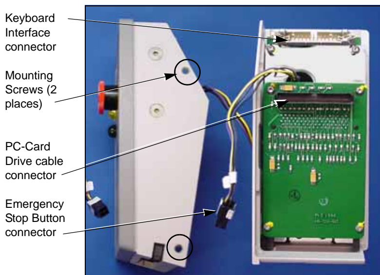
Figure 26—Location of Connectors and Screws on the Control Panel.
