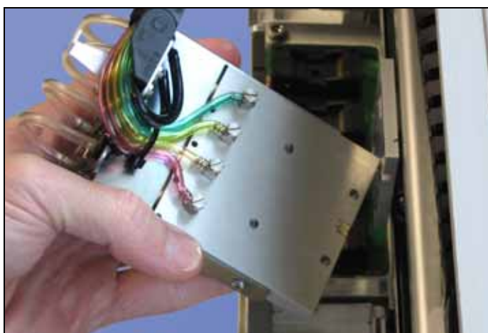
Figure 32—The four fittings on the back of the PNP Head. The PNP Head has been unbolted from the Linear Stage Module.
