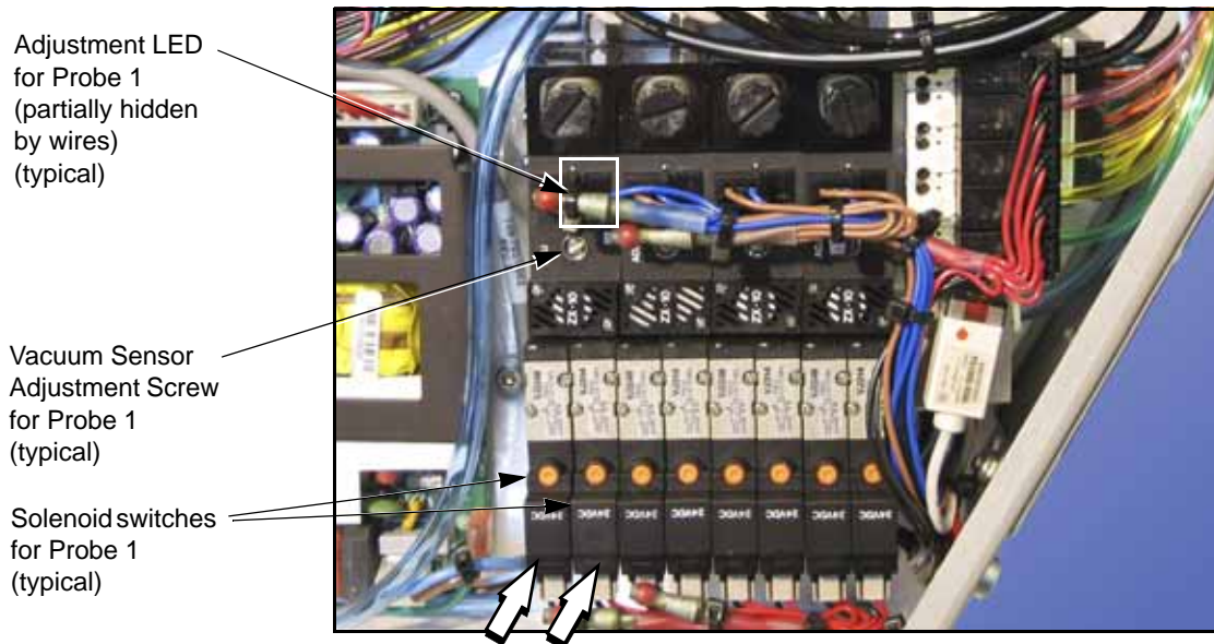
Figure 30—Pneumatic Valve Block. When the vacuum for Probe 1 is enabled, the small LED on each of the two solenoids (white arrows) for Probe 1 will be unlit.
