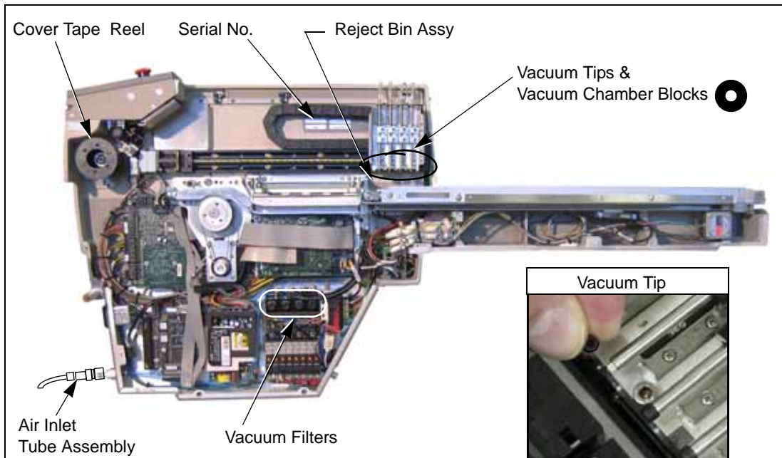
Figure 49—Parts in the Basic Spares Kit; Standard RoadRunner.
