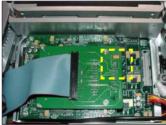
Figure 40—The Programmer: Ribbon cable J4 (not shown) is disconnected. The NVRAM Battery is on the far side of the second board down. If you had X-ray vision, you could see it where the dashed, yellow square is drawn.
