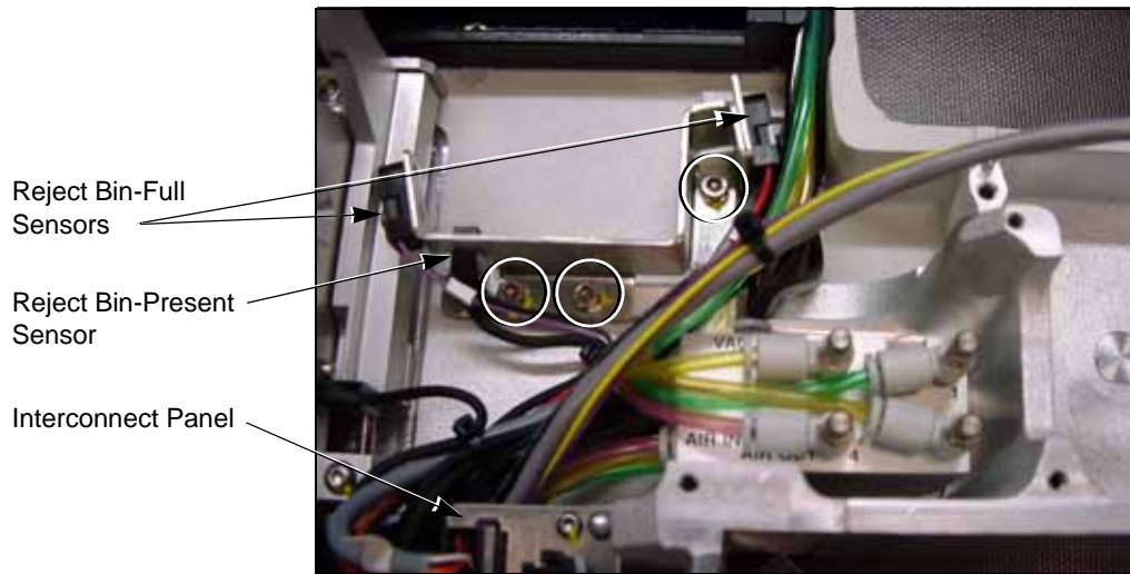
Figure 23—Reject Bin Sensors and Bracket Screw Locations.
