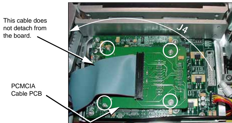
Figure 41—Ribbon cable J4 (not shown) has been disconnected from the programmer. PCMCIA-PCB screws are circled.
