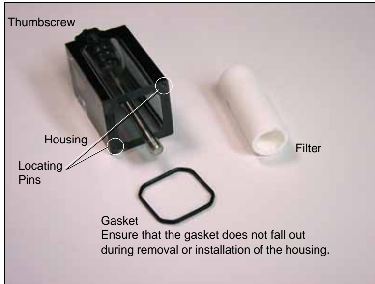
Figure 9—Vacuum Filter Components
