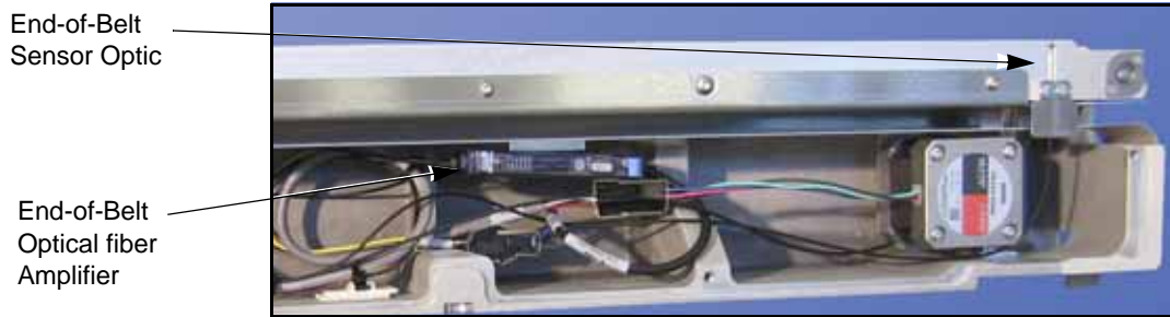
Figure 20—Retaching the End-of-Belt Sensor.
