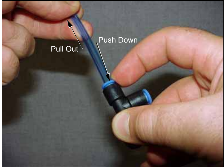
Figure 10—Disconnecting a Pneumatic Tube from the One-touch Connector
